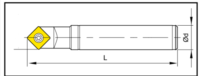
Internal Chamfering
