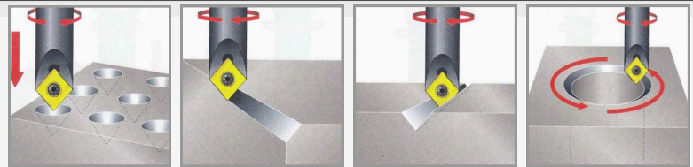
Internal Chamfering
